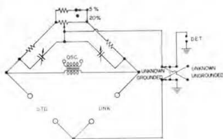
Figure 3. Elementary circuit of the bridge.
