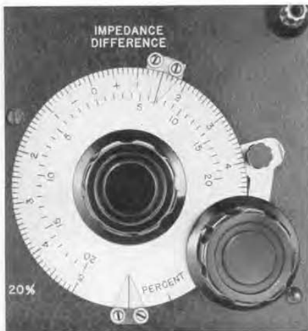
Figure 2. Close-up of the impedance-difference dial.
